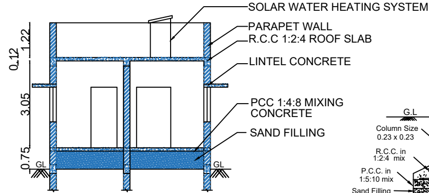
SECTION NO - "AB"
