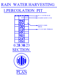
PLAN RAIN WATER HARVESTING & PERCOLATION PIT
