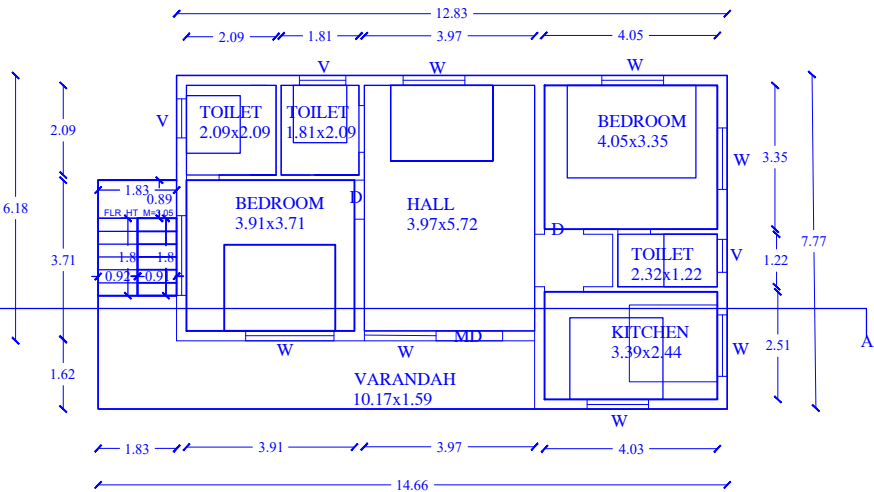
PRO. FIRST FLOOR PLAN
