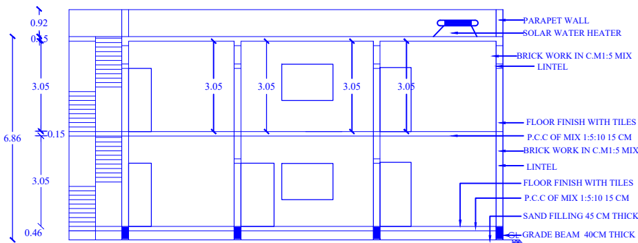
SECTION ON A-A1
