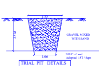
TRIAL PIT DETAILS
