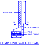
COMPOUND WALL DETAIL
