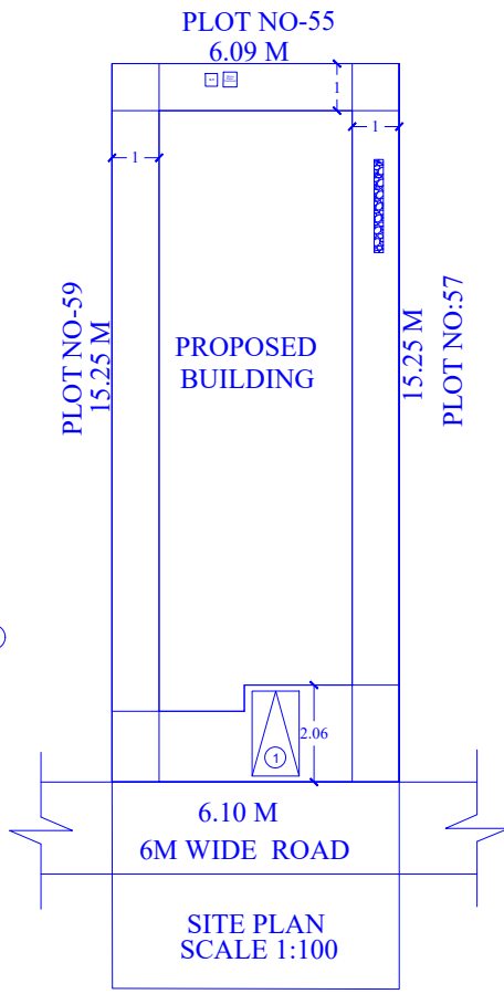
PLAN
