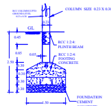
FOUNDATION DETAILS Scale 1:50
