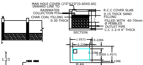
RAINWATER HARVESTING
