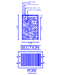
RAIN WATER HARVESTING PERCOLATION BED
