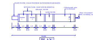
WASTE WATER RECYCLING SYSTEM
