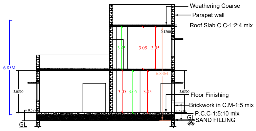
CROSS SECTION ON AB
