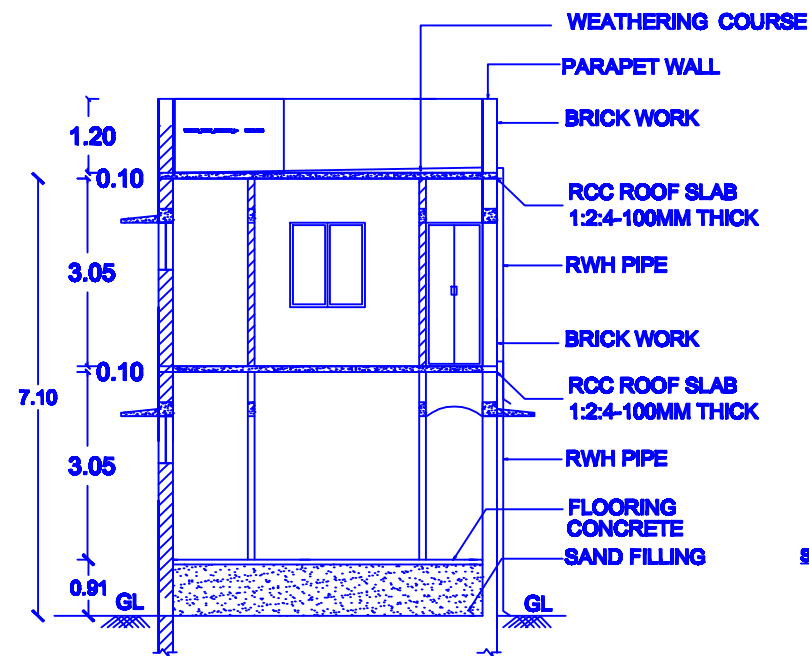
SECTION X-Y
