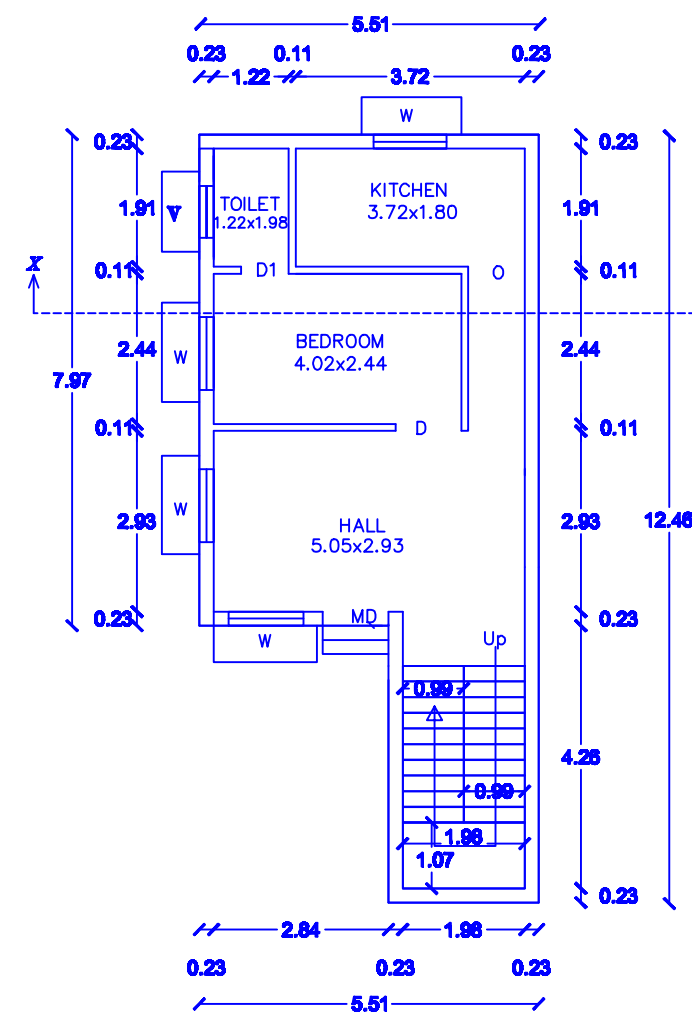
GROUN FLOOR PLAN
