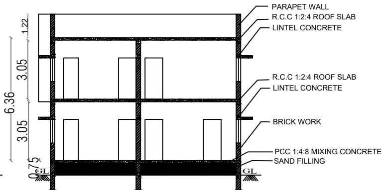
SECTION - "AB"
