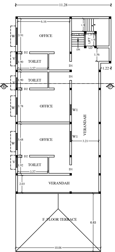
PRO- SECOND FLOOR PLAN
