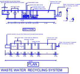
WASTE WATER RECYCLING SYSTEM
