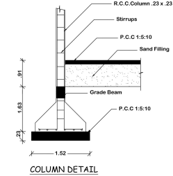
COLUMN DETAIL
