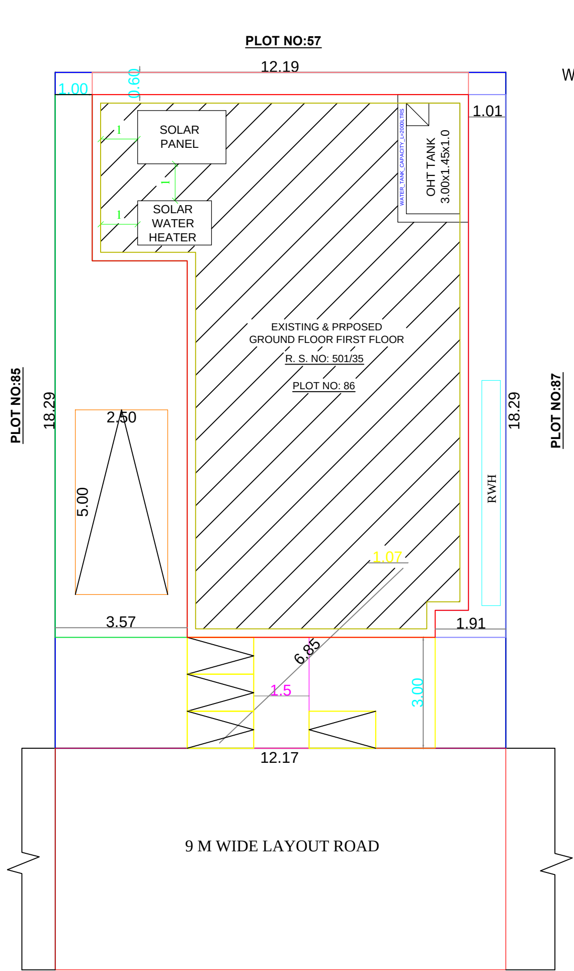
SITE PLAN
