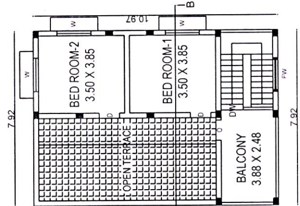
PRO. FIRST FLOOR PLAN
