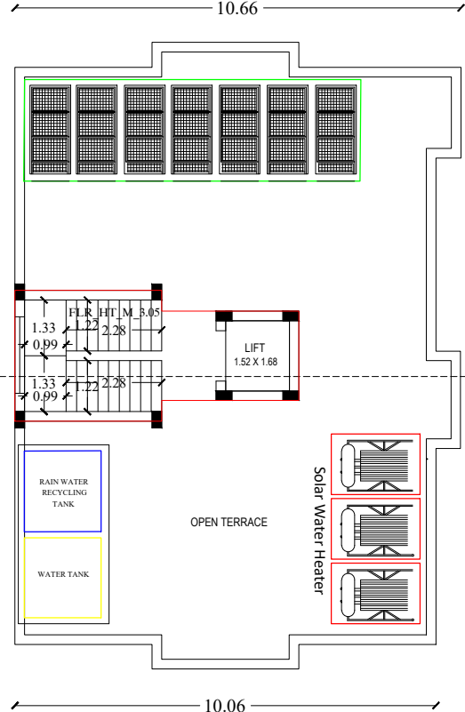
TERRACE PLAN
