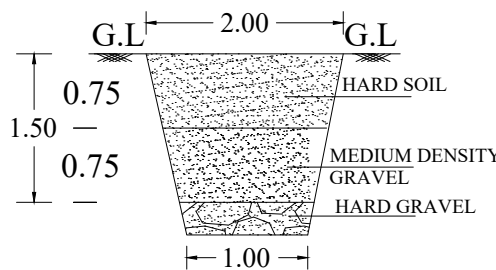
TRIAL PIT
