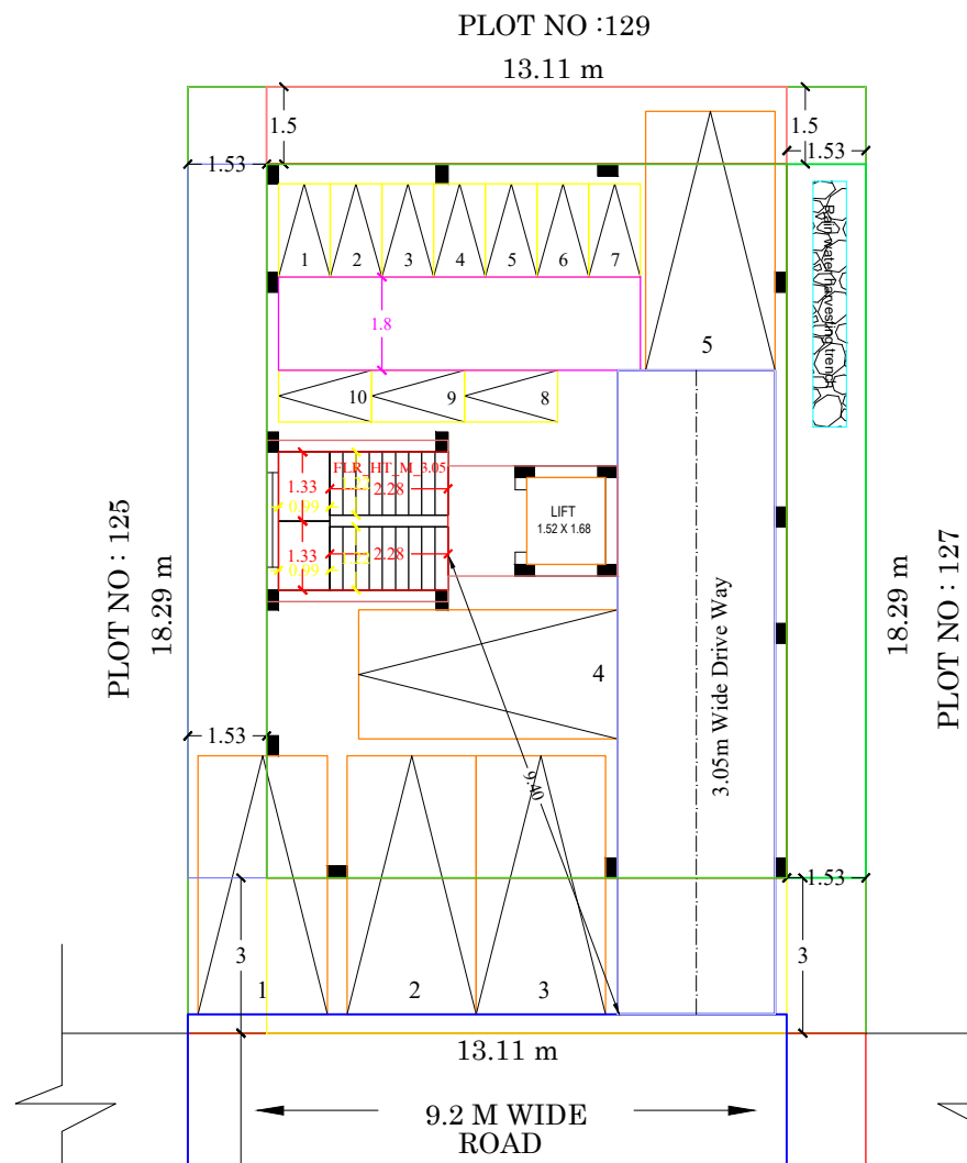
SITE CUM STILT FLOOR PLAN
