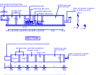
WASTE WATER RECYCLING SYSTEM
