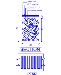
RAIN WATER HARVESTING PERCOLATION BED
