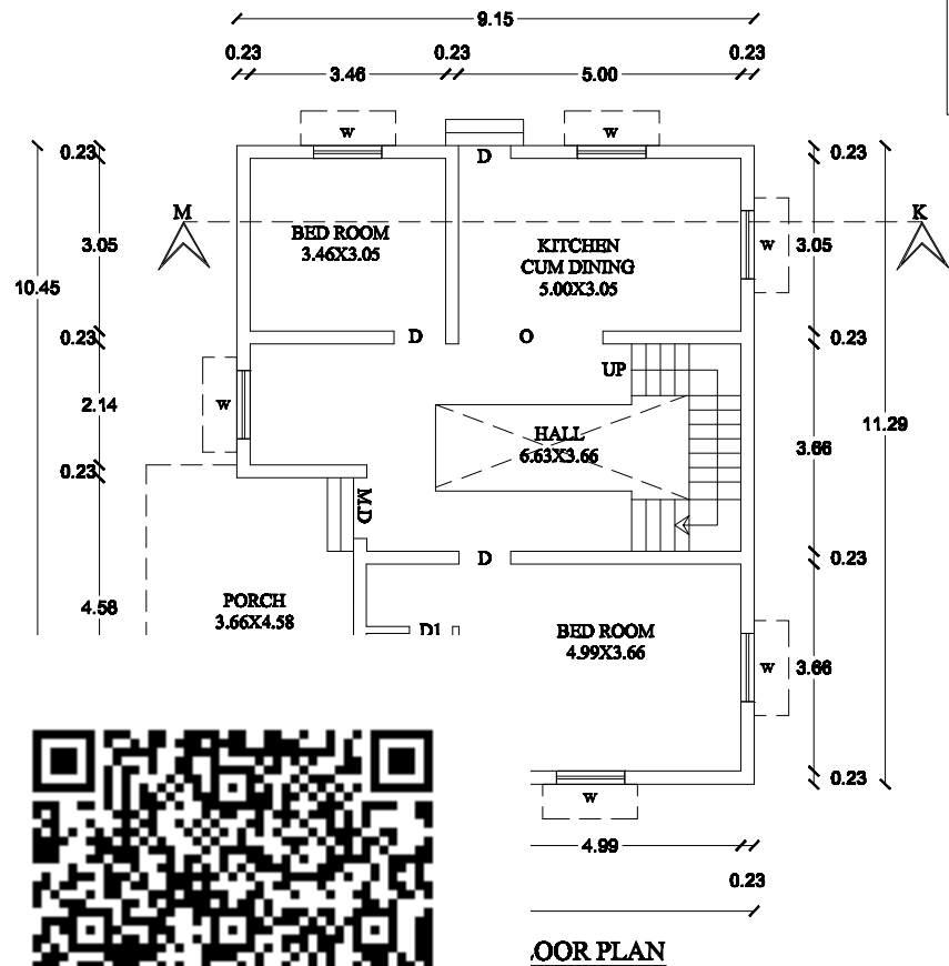
FLOOR PLAN
