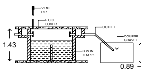
SEPTIC TANK & D-TRENCH DETAILS [ NOT TO SCALE ]
