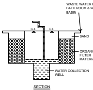
PLAN AND SECTION OF ORGANIC FILTRATIONS SUMP WITH COLLECTION WELL
