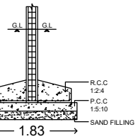
COLUMN DETAILS [ NOT TO SCALE ]
