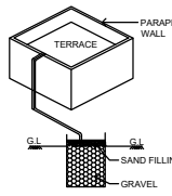
COLLECTION SUMP FOR HARVESTING FOR TERRACE
