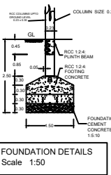
FOUNDATION DETAILS Scale: 1:50
