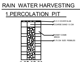
RAIN WATER HARVESTING 1. PERCOLATION PIT
