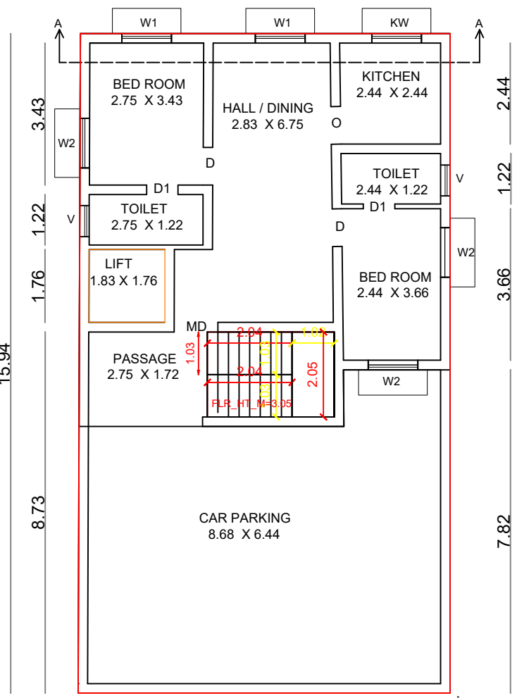
EXI. GROUND FLOOR PLAN
