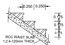
STAIR CASE STEPS SCALE 1:25
