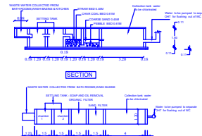
WASTE WATER RECYCLING SYSTEM
