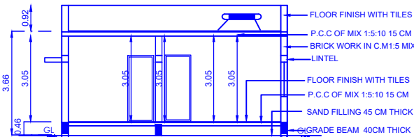
SECTION ON A-A1
