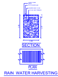
RAIN WATER HARVESTING PERCOLATION BED
