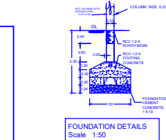
FOUNDATION DETAILS Scale: 1:50
