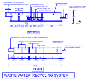
WASTE WATER RECYCLING SYSTEM
