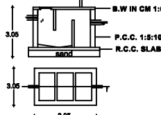
Septic tank detail
