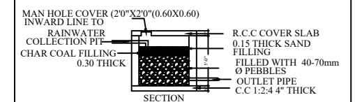
SECTION
