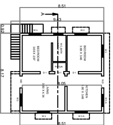
PROPOSED GROUND FLOOR
