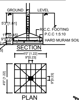
COLUMN SIZE = 0'9" X 0'9"
