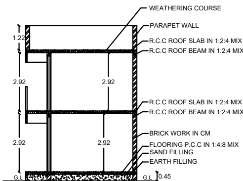
SECTION ON-AB
