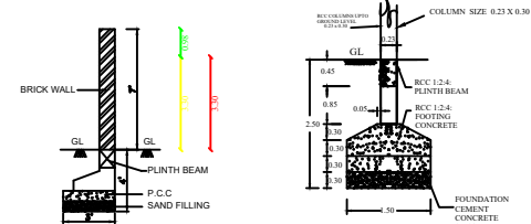
FOUNDATION DETAILS Scale 1:50
