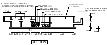
WASTE WATER RECYCLING SYSTEM
