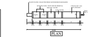
WASTE WATER RECYCLING SYSTEM
