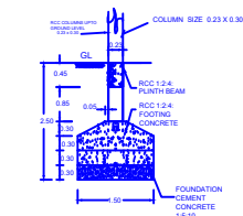
FOUNDATION DETAILS Scale 1:50
