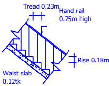
STAIR DETAILS
