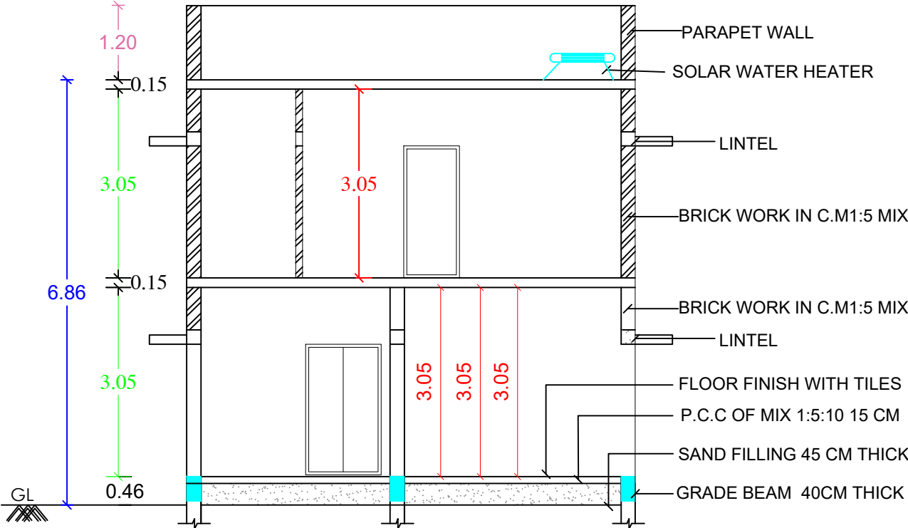
SECTION-A-A1
