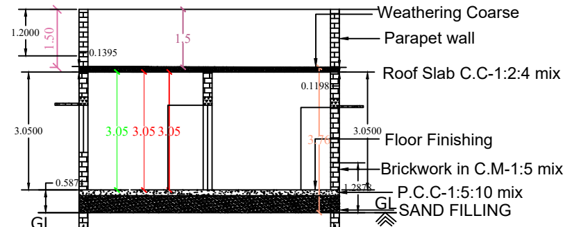
CROSS SECTION ON XX
