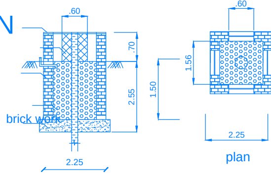
RAIN WATER HARVESTING PIT
