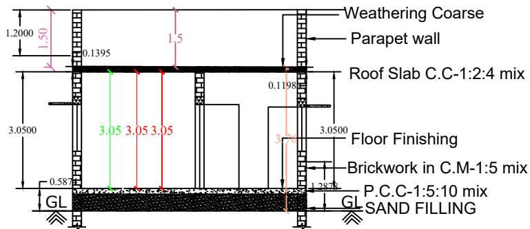
CROSS SECTION ON XX
