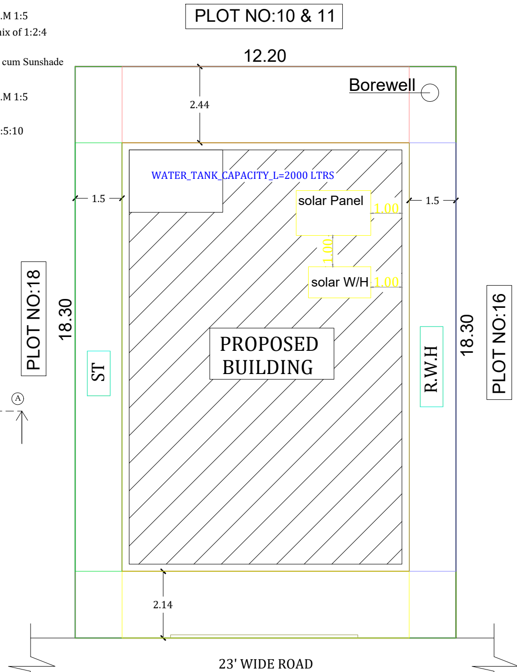
SITE PLAN
