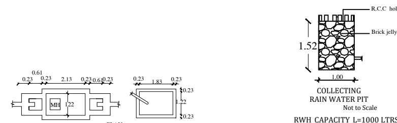
COLLECTING RAIN WATER PIT
