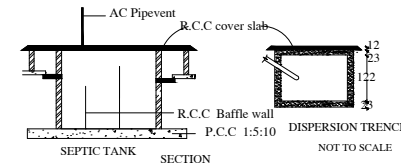
AC PIPEVENT
