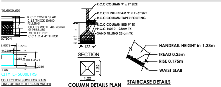
COLUMN DETAILS PLAN STAIRCASE DETAILS
