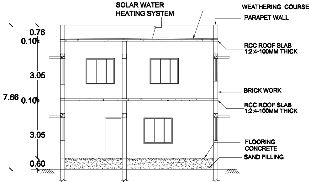
SECTION ON RM
