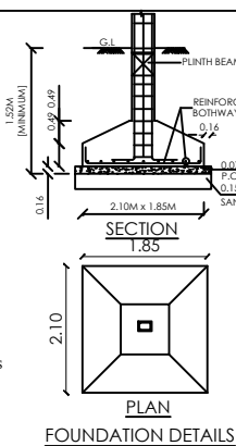
FOUNDATION DETAILS
