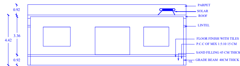
SECTION-AB
