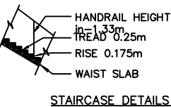
STAIRCASE DETAILS
