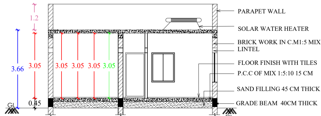
SECTION- AA1
