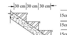
RCC WAIST SLAB 1:2:4-120mm THICK STAIR CASE STEPS SCALE 1:25
