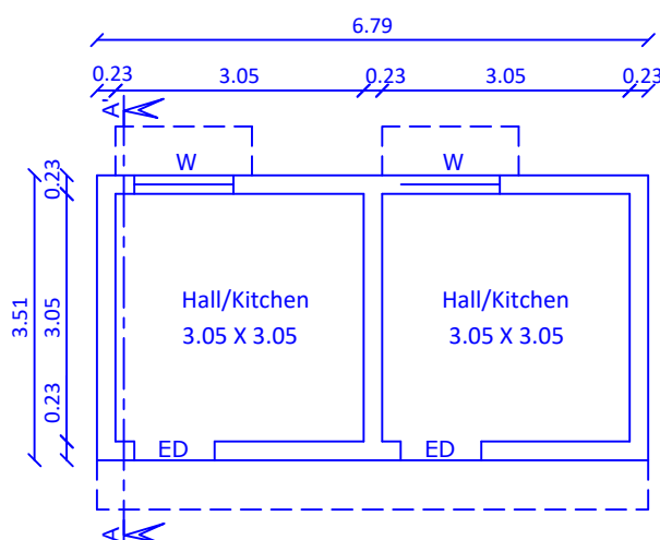
LABOUR SHED PLAN
