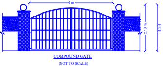
COMPOUND GATE
