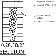
SECTION PLAN
