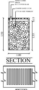
SECTION PLAN RAIN WATER HARVESTING PERCOLATION BED
