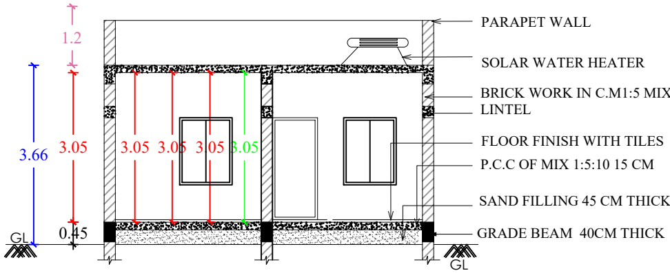
SECTION- AA1
