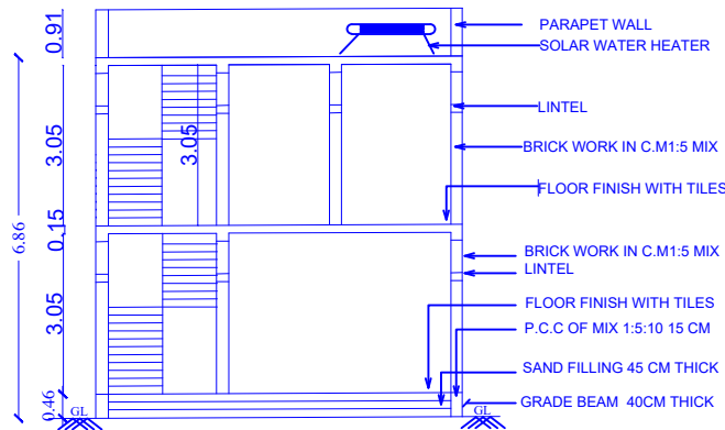
SECTION-AB
