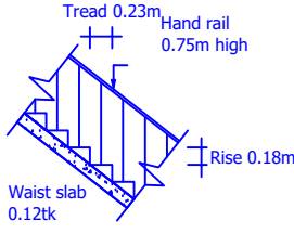
STAIR DETAILS
