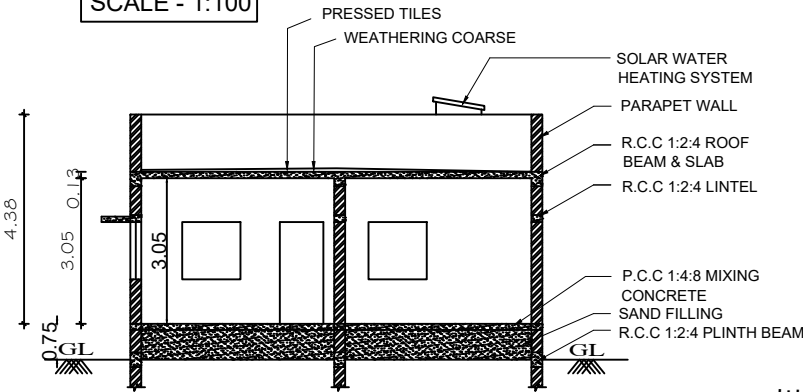
SECTION "A-B"
