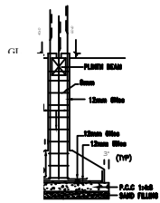
FOUNDATION DETAILS SCALE : 1:50.
