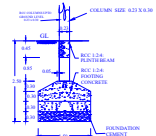
FOUNDATION DETAILS Scale 1:50
