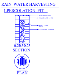
RAIN WATER HARVESTING PERCOLATION PIT
