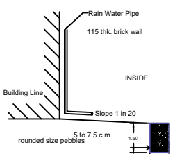
Percolation pit
