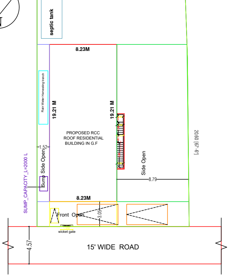
SITE PLAN [1:100]
