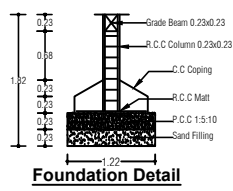
Foundation Detail
