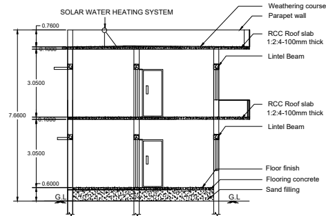
SECTION ON MK
