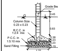
COLUMN DETAILS NOT TO SCALE
