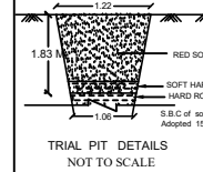
TRIAL PIT DETAILS NOT TO SCALE
