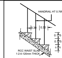
STAIR CASE DETAILS SCALE 1:25
