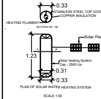
SCALE 1:50
