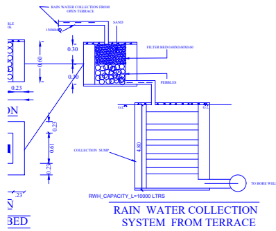
RAIN WATER COLLECTION SYSTEM FROM TERRACE
