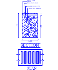
RAIN WATER HARVESTING PERCOLATION BED
