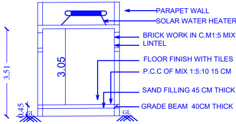
SECTION-AB
