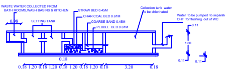
SECTION
